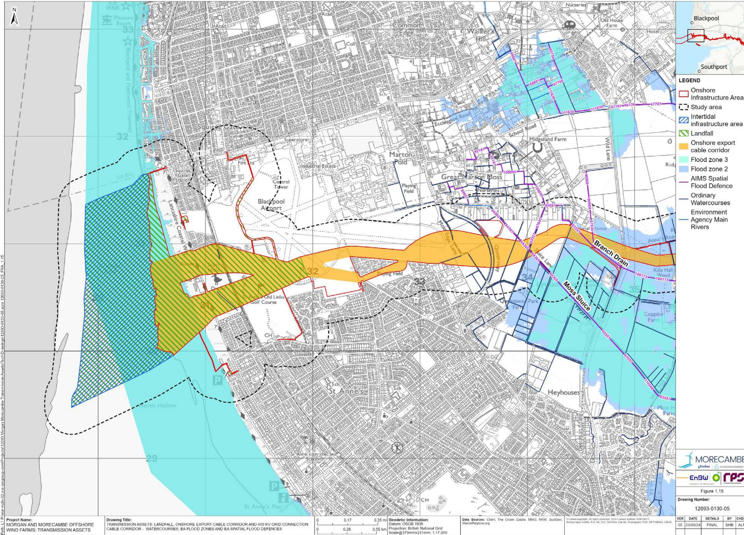
Figure 1.15a: Transmission Assets: landfall, onshore export cable corridor and 400 kV grid connection cable corridor - Watercourses, EA Flood Zones and EA Spatial Flood Defences
